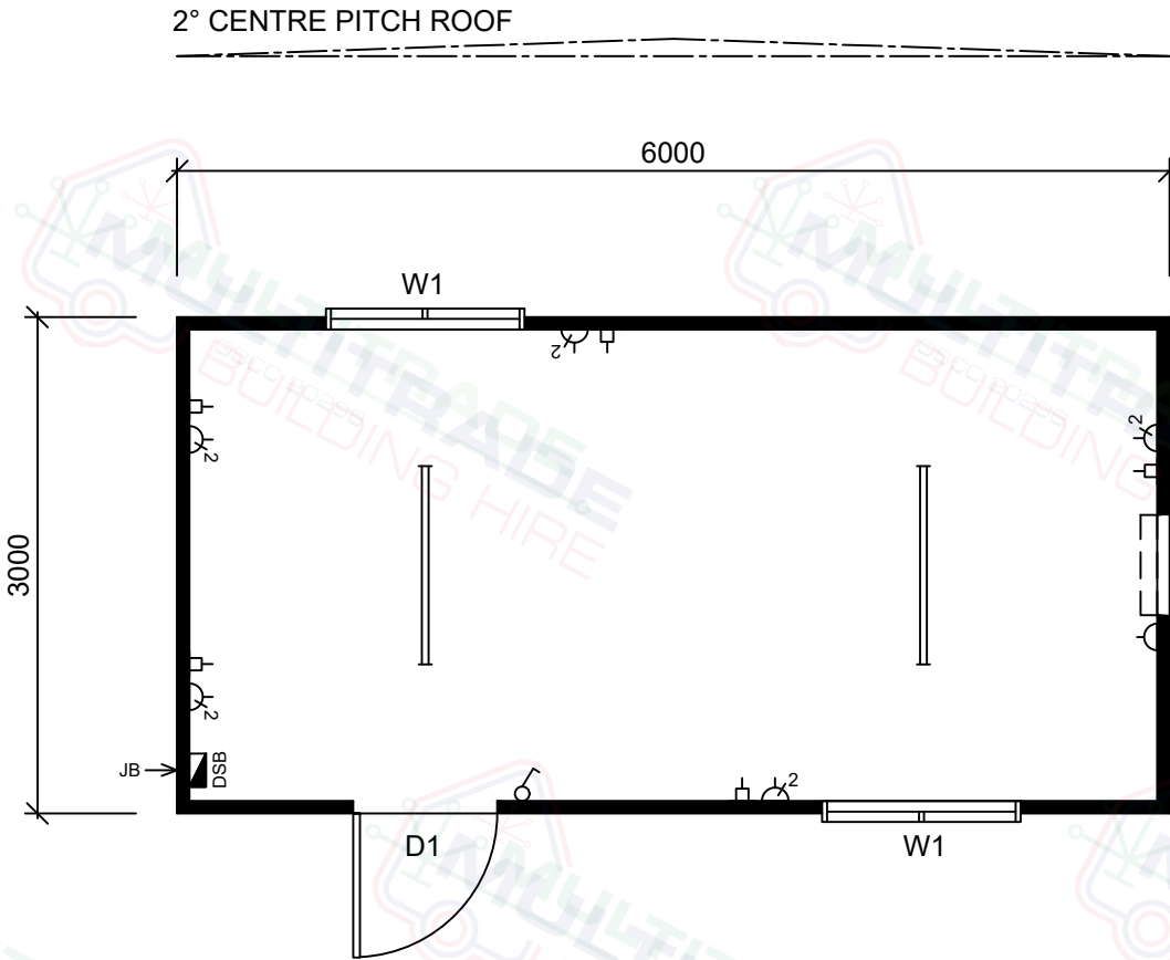
6.0x3.0m Office - Floor Plan
